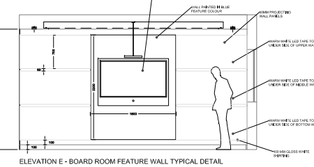
ELEVATION E - BOARD ROOM FEATURE WALL TYPICAL DETAIL
