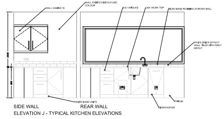
SIDE WALL ELEVATION J - TYPICAL KITCHEN ELEVATIONS
