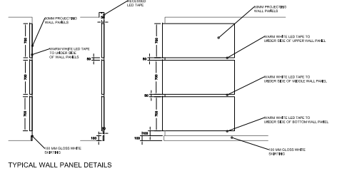
TYPICAL WALL PANEL DETAILS
