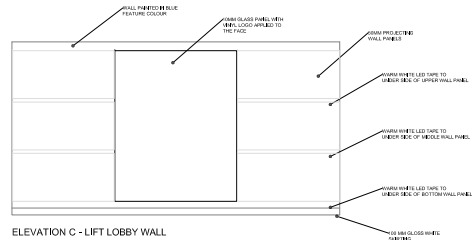
ELEVATION C - LIFT LOBBY WALL
