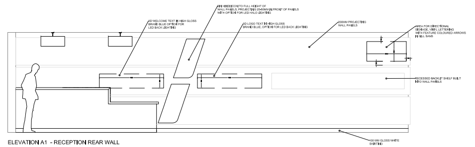
ELEVATION A1 - RECEPTION REAR WALL
